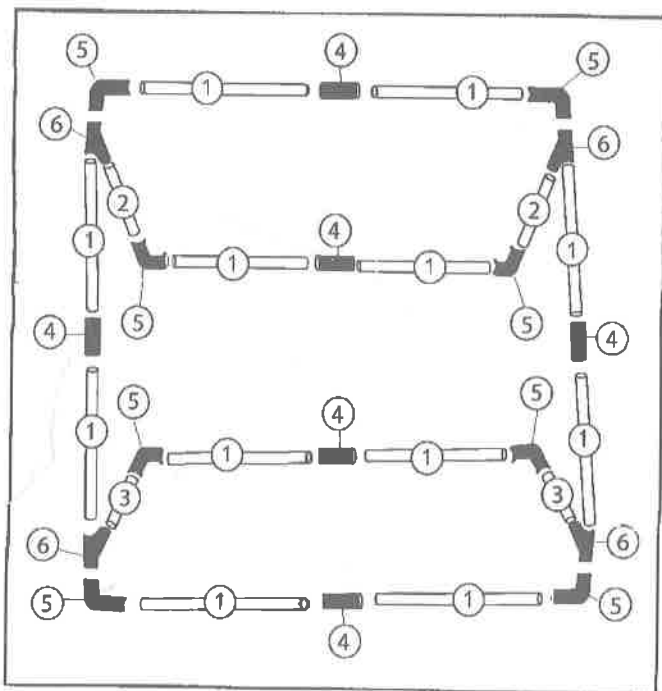
Diagram 1. Frame Assembly
